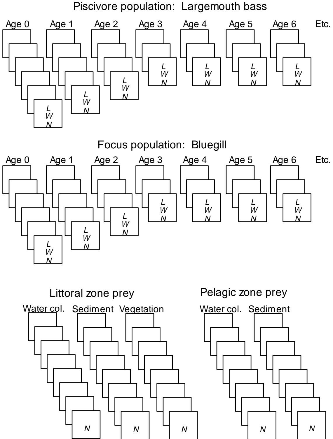
Figure 1.—The components of LakeMod include a population of piscivores, such as largemouth bass; the focus population of bluegill; and five habitat types containing fixed sizes of invertebrate prey. The total number of “individual” fish in the model may be several hundred, each with three state variables: L = length, W = weight, and N = number of identical fish in the lake represented by the modeled “individual.” For each of the eight fixed size categories of prey in a habitat type, the state variable N = number of prey per unit area or volume.
