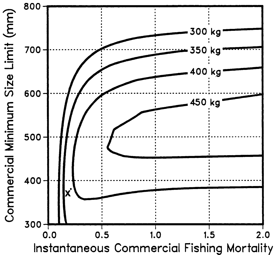
Figure 9. Yield isopleth diagram for commercial yield per 1000 recruits of channel catfish from Saginaw Bay, 1985. Instantaneous natural and sport fishing mortality rates were 0.19 and 0.05, respectively. The commercial fishery was operating a point x in 1985.
