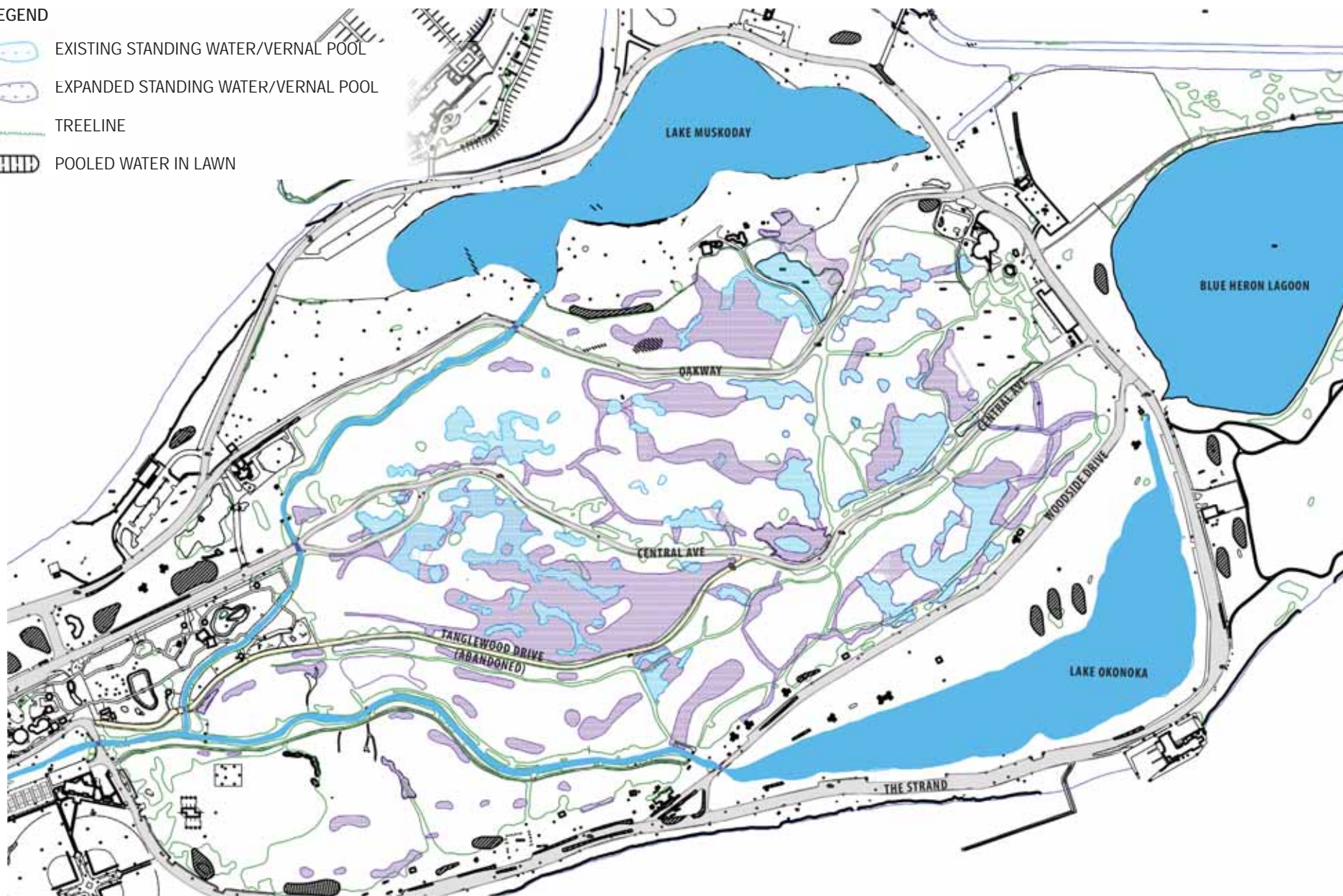
Figure 4. Forest Hydrology-Pools
