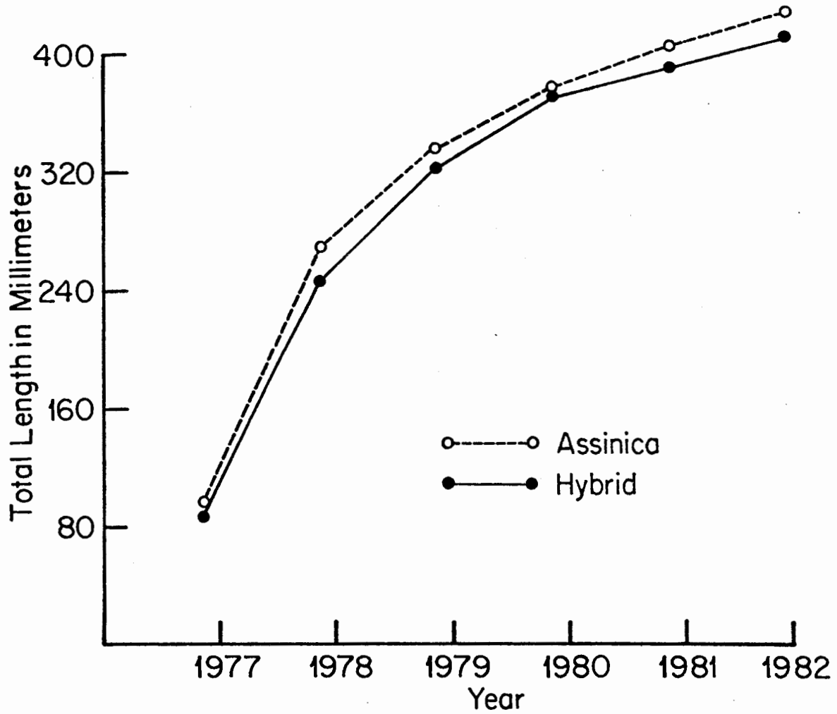
Figure 4. Growth in total length (mm) of Assinica and hybrid stream brook trout from pooled data for six experimental waters.
