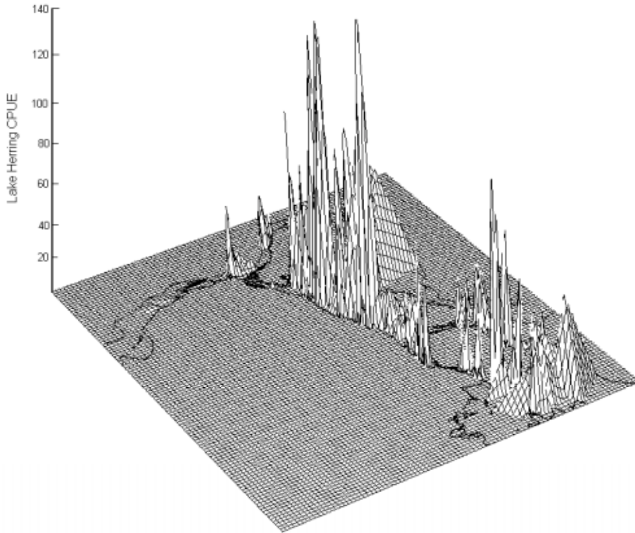
Appendix 1.—Number of all lake herring (sexes and maturity levels combined) per 91.4 m of gill net (CPUE) captured at sampling locations in 1993 through 1996, St. Marys River.
