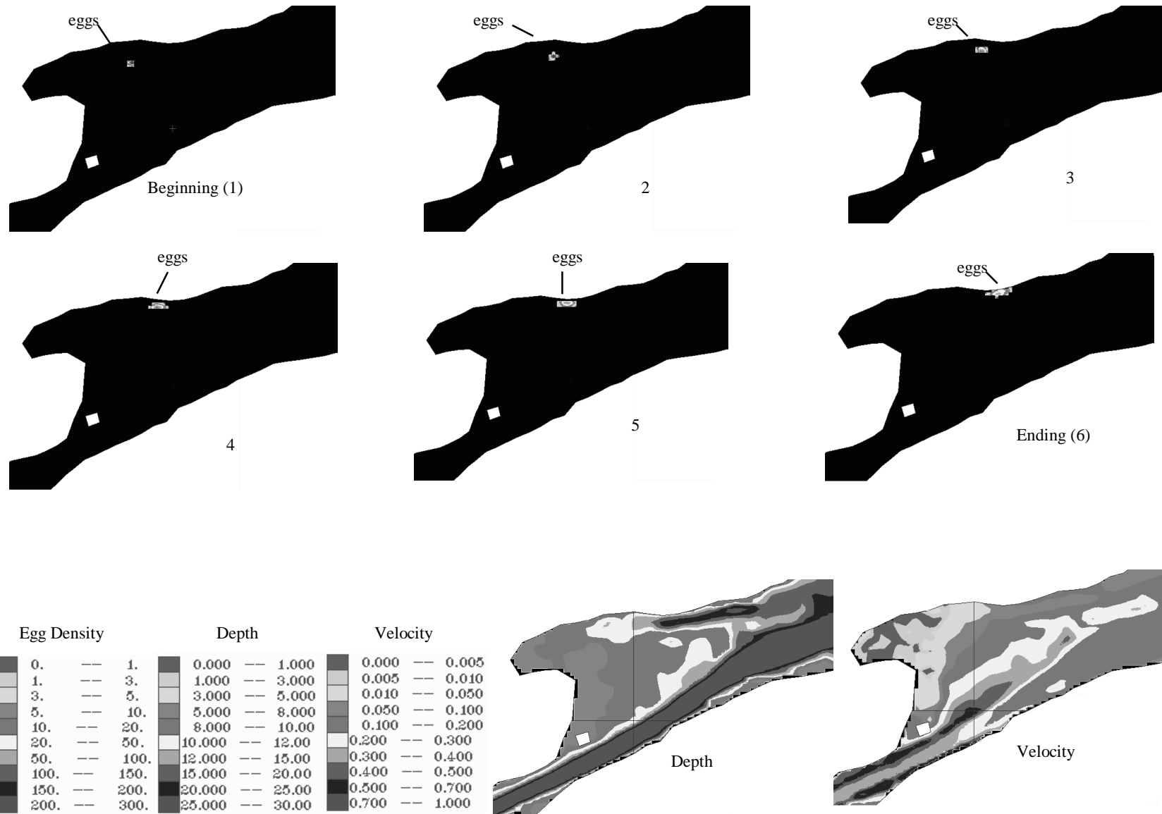
Figure 7. Six hour egg transport prediction for the Baie de Wasai vicinity (a high importance area). Distance traveled by egg mass was 1,200 m. Egg density is in eggs/m 2 , velocity in m/s, and depth in m.
