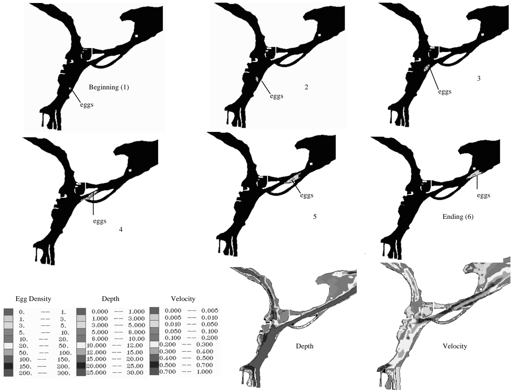
Figure 8.—Six hour egg transport prediction for the Locks area (a low importance area). Distances traveled by egg mass was 9,000 m. Egg density is in eggs/m 2 , velocity in m/s, and depth in m.
