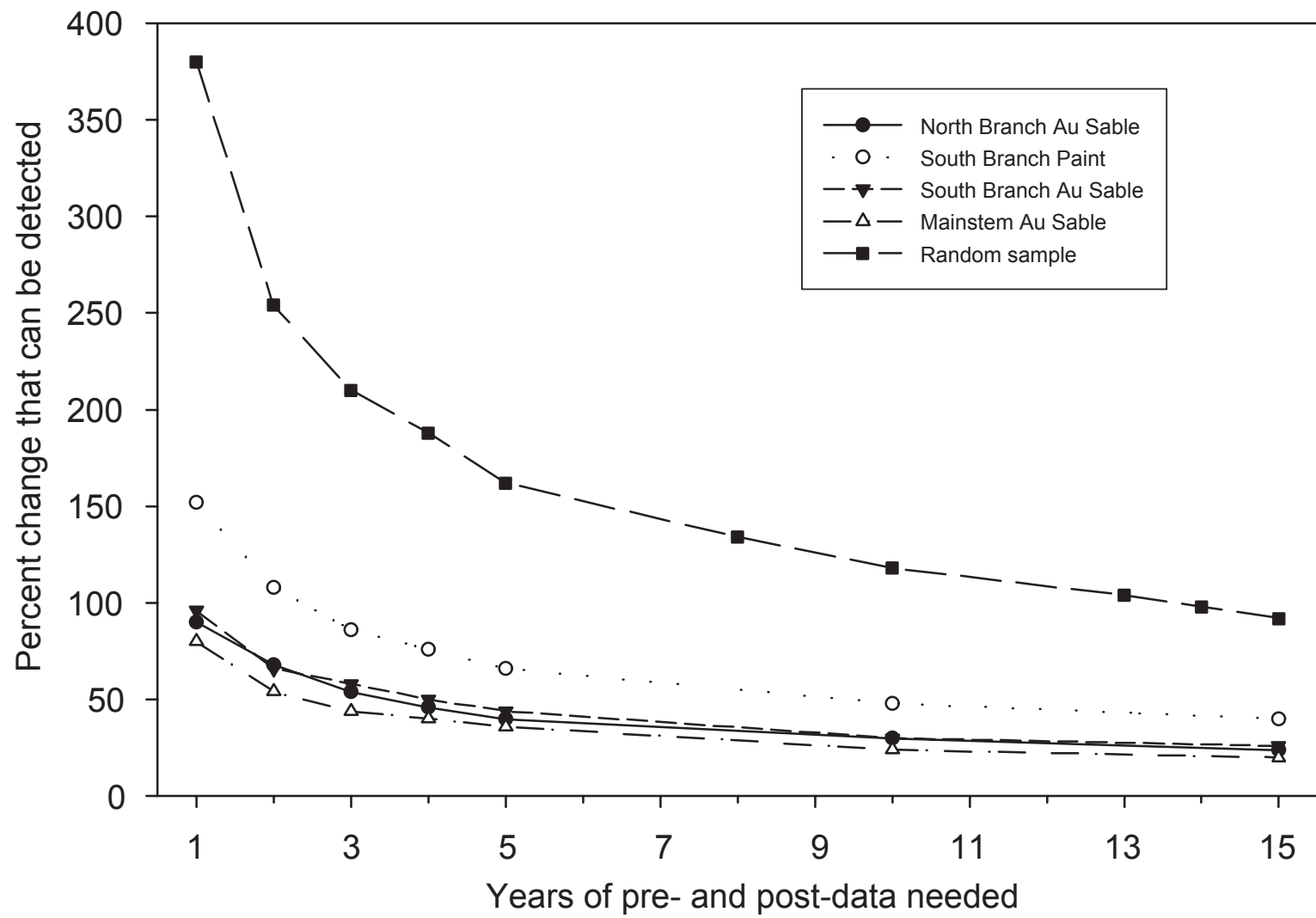
Figure 26.1.—Brown trout trend detection ability at fixed vs. random sites.
