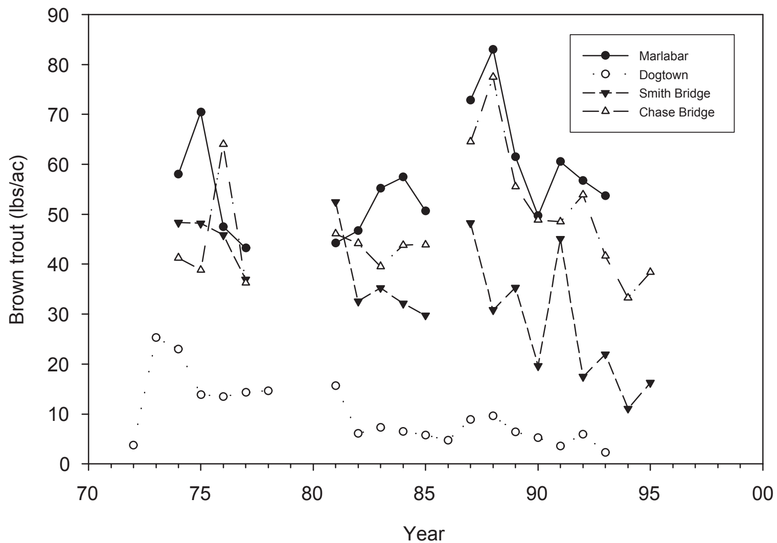
Figure 26.2.—Consistent differences and similar trends among sites in the South Branch Au Sable River.
