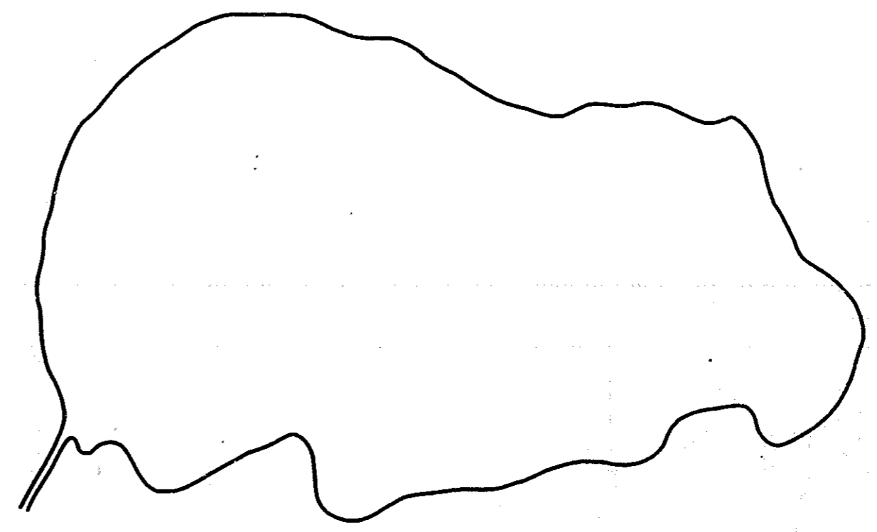
Aquatic Vegetation Map
