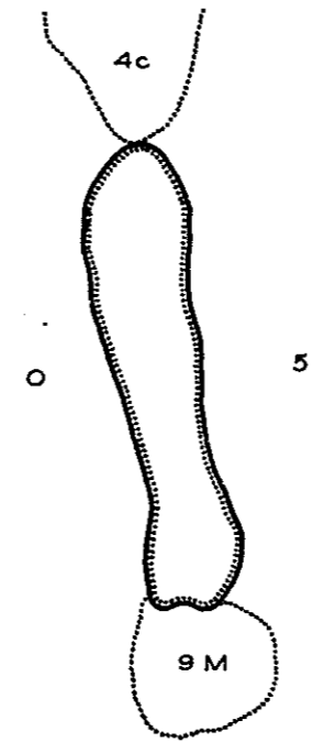
Cover Type And Lake Bottom Soil Type Map
