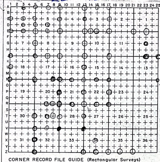
CORNER RECORD FILE GUIDE (Rectangular Surveys)
