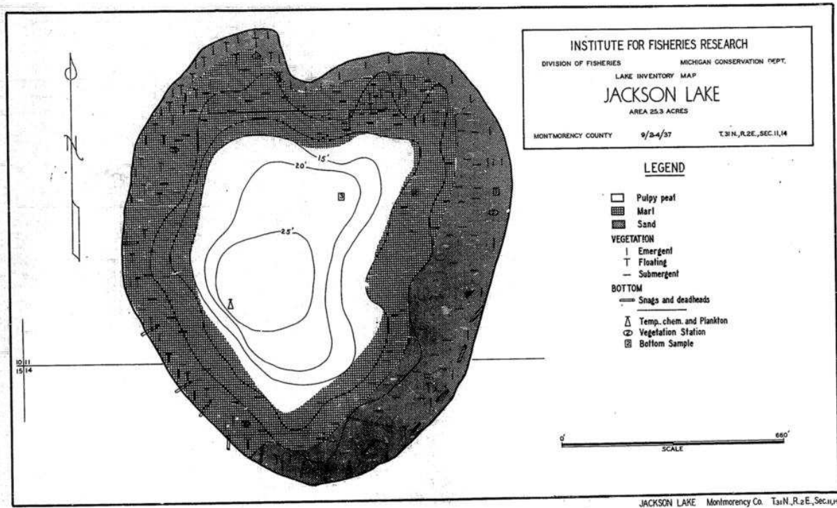
Figure 2. Jackson Lake bathymetric map.
