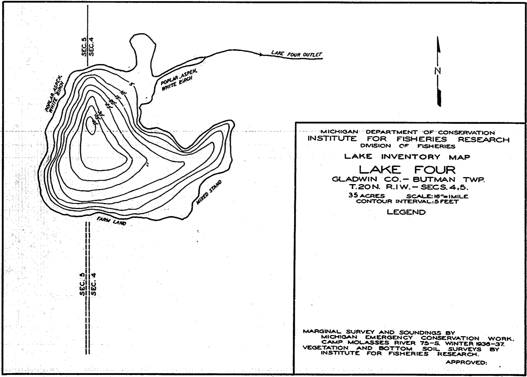
LAKE FOUR GLADWIN CO. T.20N. R.1W. SECS. 4,5
